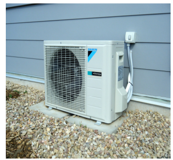
Our rarely used heat pump COP 5 0.8kW electricity in 4kW heat out
